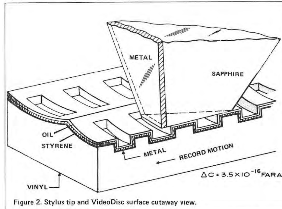
Figure 1. Stylus tip and VideoDisc surface.
